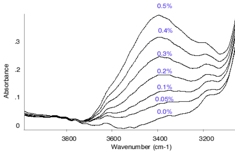
IR spectrum of a mineral oil contaminated with water (0 – 0.5 vol. %)
